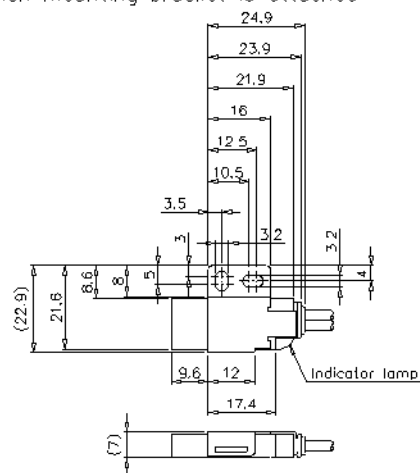
When mounting bracket is attached
