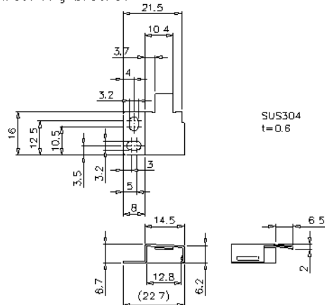
Mounting bracket
